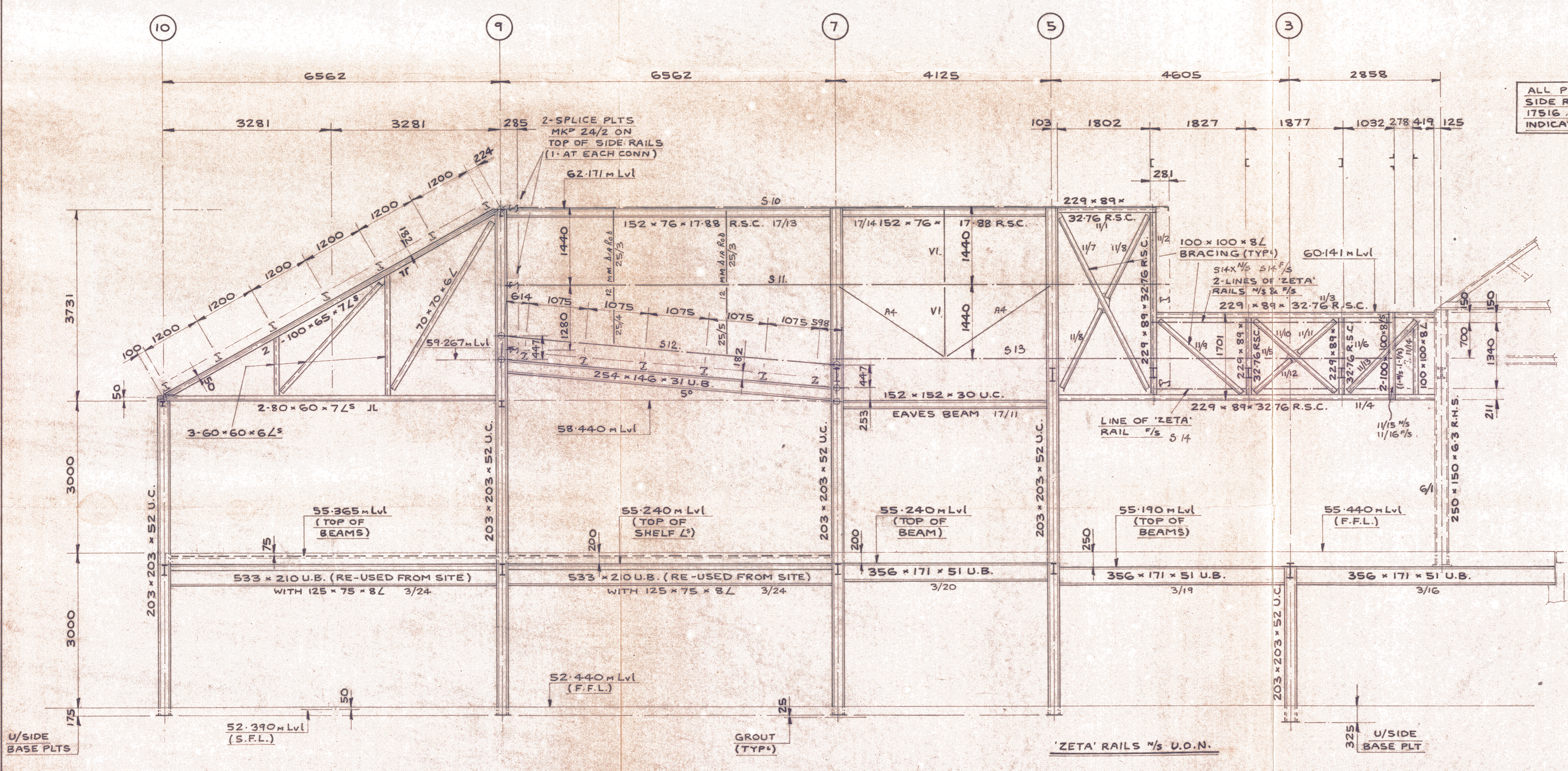
CROSS SECTION AT GRID LINE Aa
