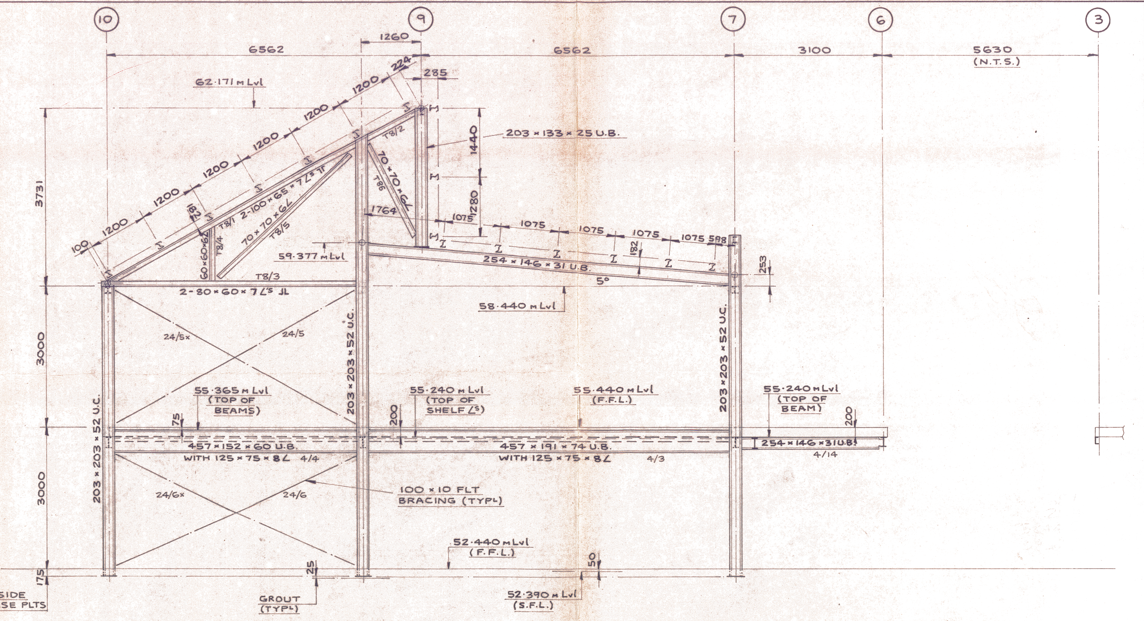
ELEVATION/CROSS SECTION AT LINE Ea
