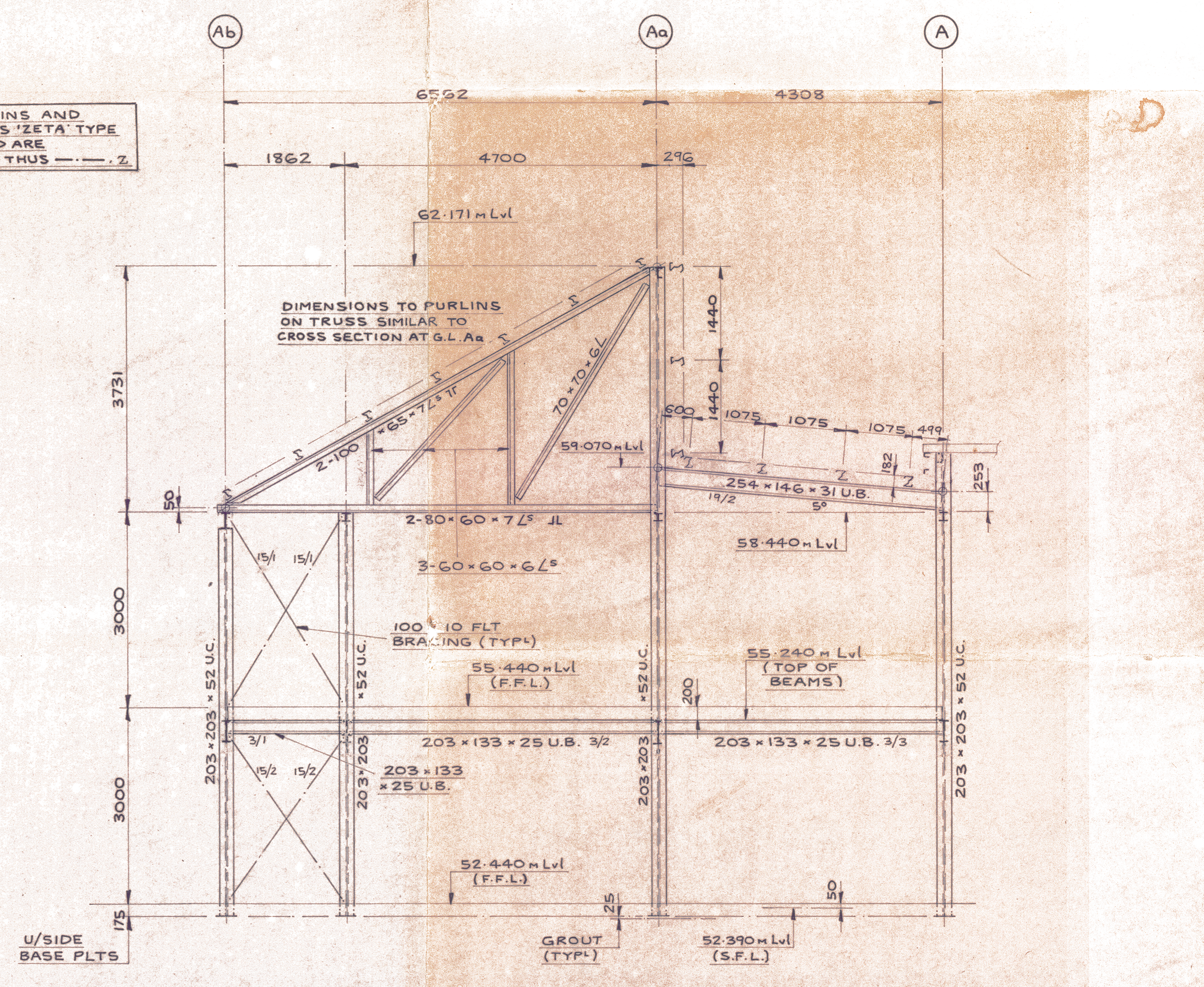
CROSS SECTION AT GRID LINE 5
