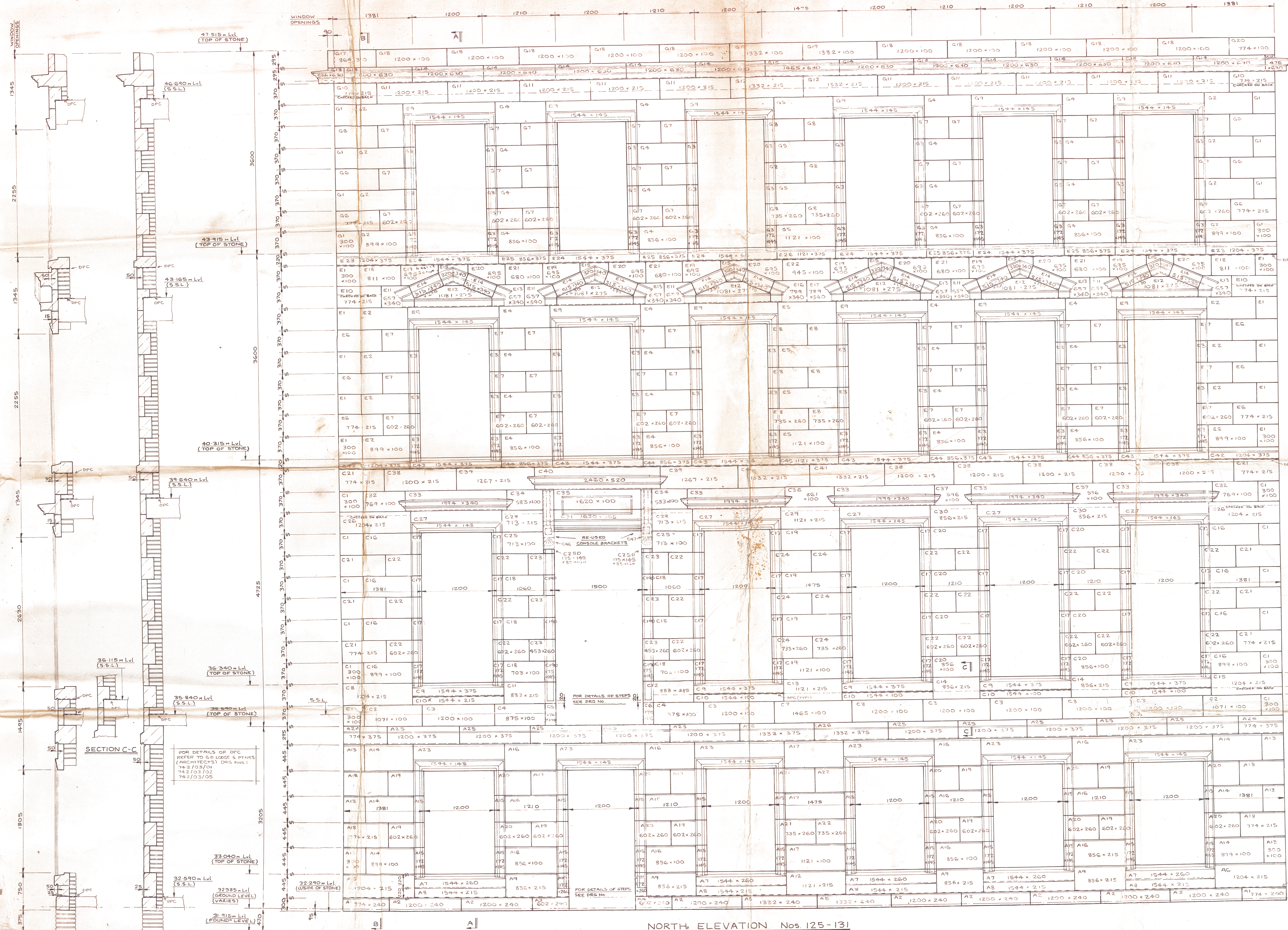
NORTH ELEVATION Nos. 125-131
